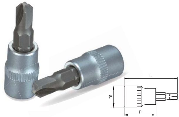
3/8"DR. MORTORQ SURPER® BIT SOCKETS
