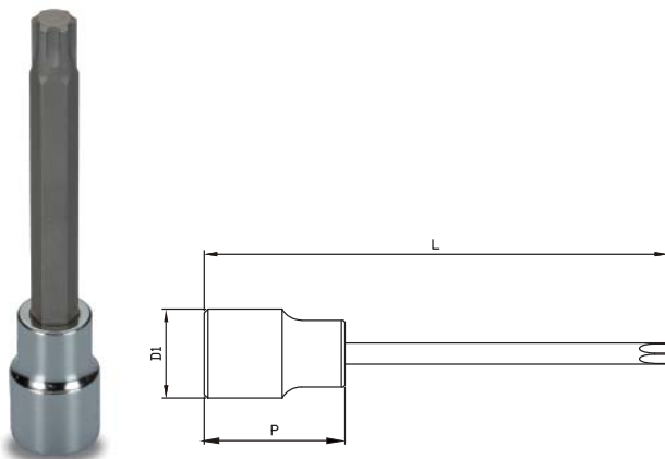
1/2"DR. VW/AUDI HEAD BOLT BIT SOCKET
