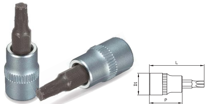
3/8"DR. TORXPLUS® BIT SOCKETS
